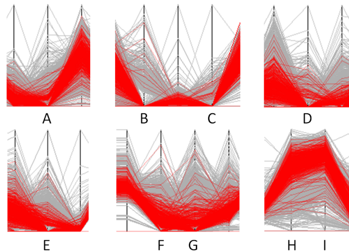
Figure 11: A meta-pattern consisting of nine discriminating text features (discriminating in terms of an unusual behavior (compared to the gray colored news)). A: unlike coordinated phrase; B: direct question; C: inverted yes/no question; D: seem/appear verb; E: conjunction phrase; F: particle; G: pronoun; H: function word; I: general service word. It is interesting that only the last ones H & I have in general a higher value than the other news belonging to Citigroup (see Figure 12). No filters are applied when we are taking the screenshots. Only the duration of the sequential pattern is limited to 60 minutes.
