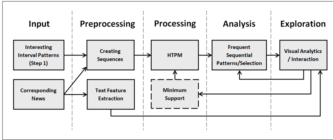
Figure 5: The sequential temporal pattern generation and exploration pipeline.
